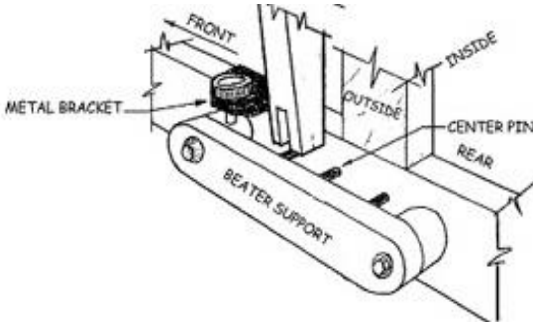
Figure 33 - Beater Support
