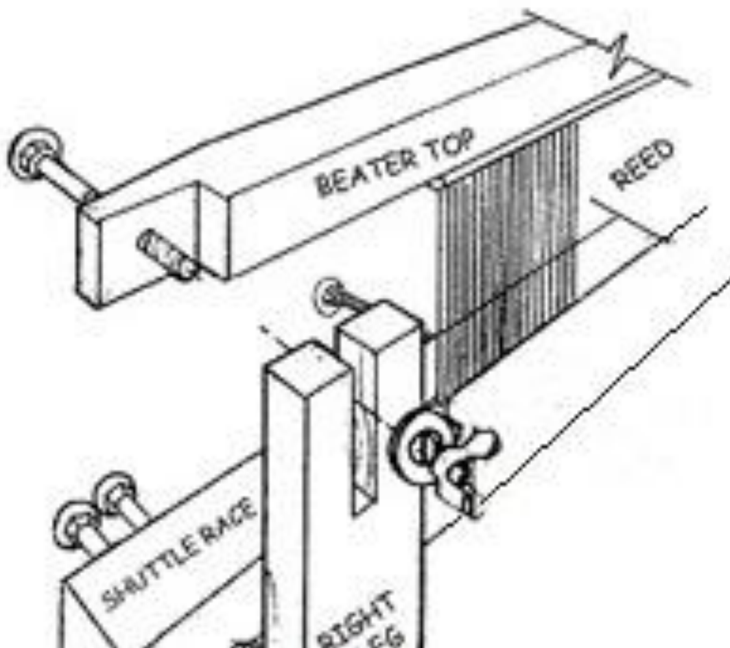
Figure 35 - Beater Top
