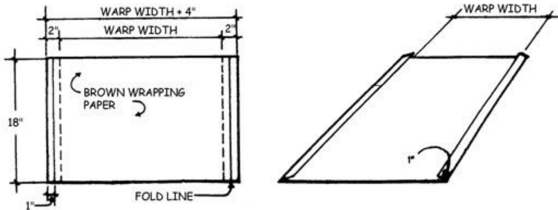
Figure 58 - Prepared Paper with Folded Edge
