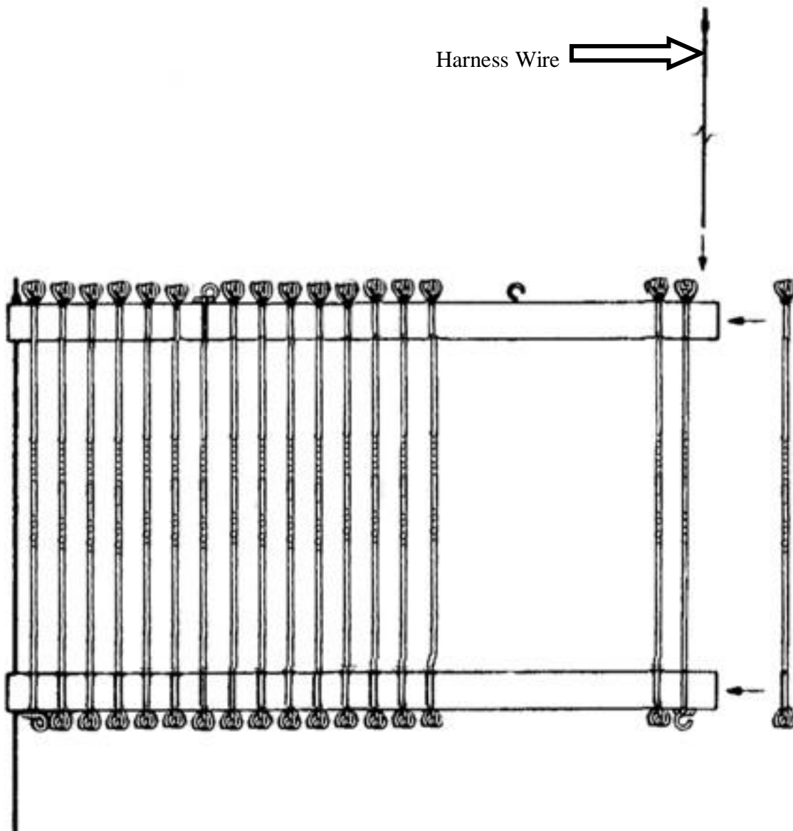
Figure 28 - Texsolv Heddle Installation
