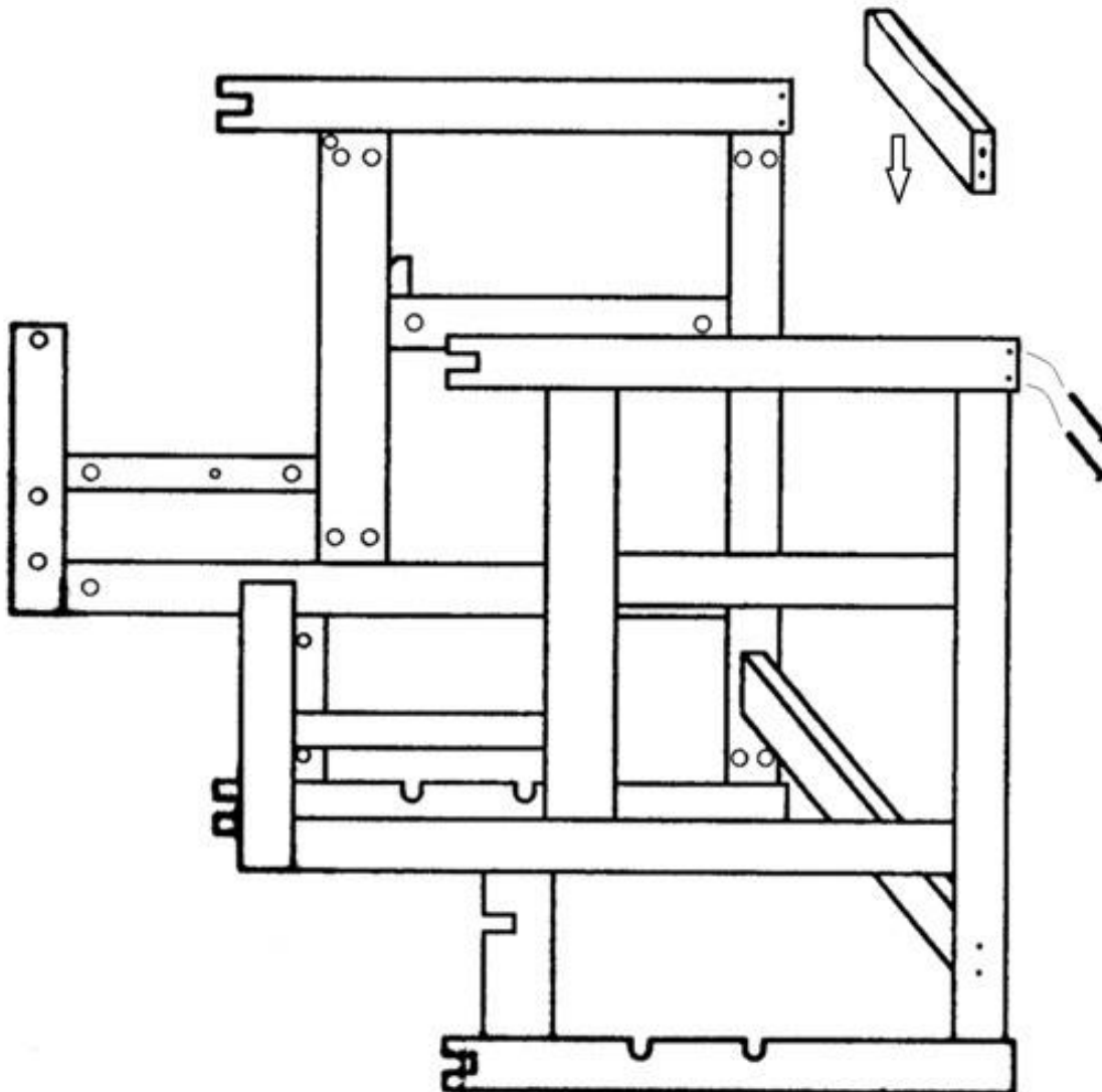
Figure 14 - Frames on Rear Verticals
