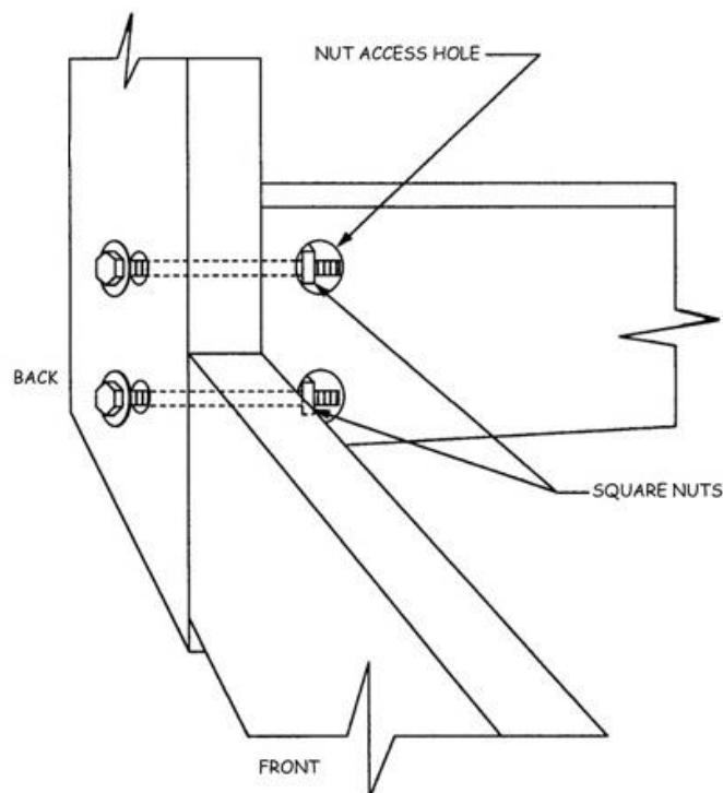
Figure 1 - Inserting Nuts
