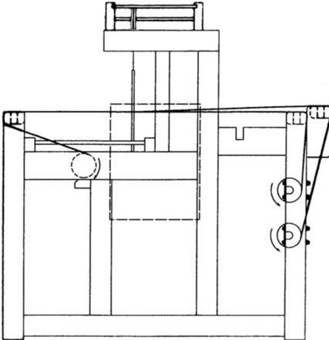
Figure 73 - Warp Routing
