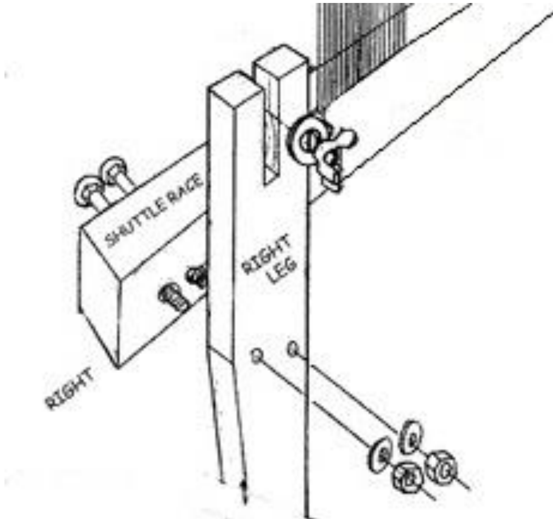
Figure 34 - Beater Leg
