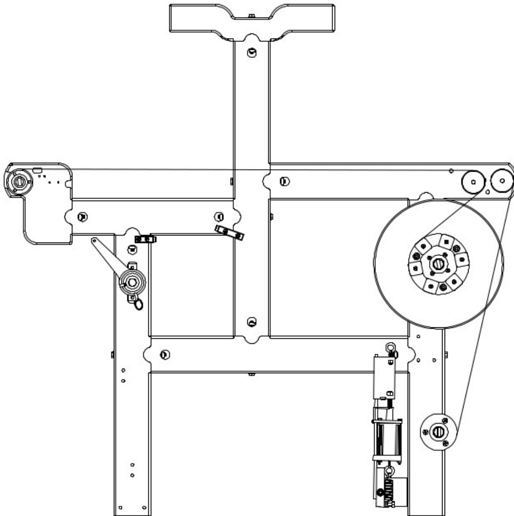
Figure 89 – Warp routing
