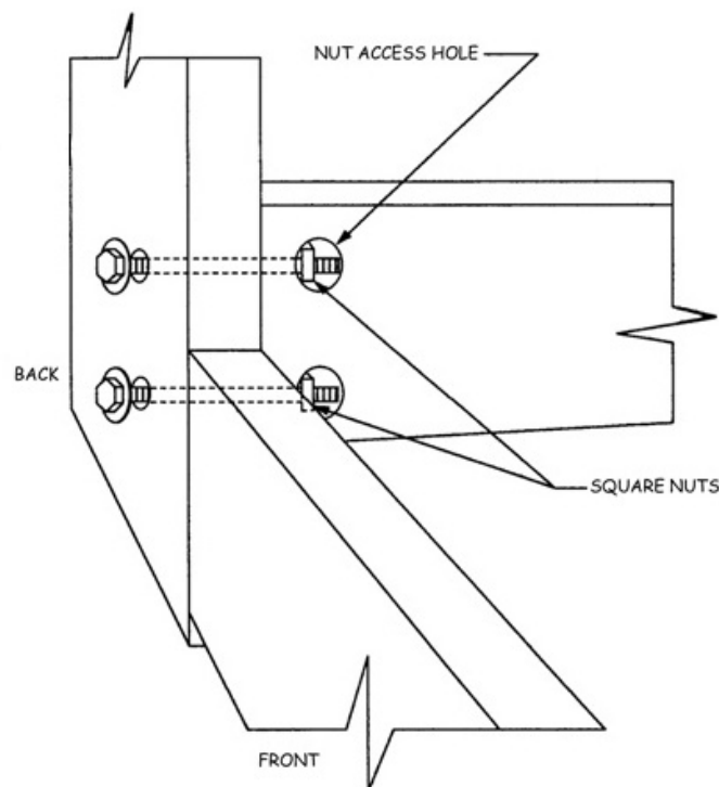
Figure 7 - Inserting Nuts
