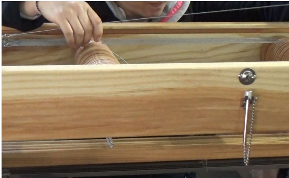
Figure 29 - Placing top harness cables
