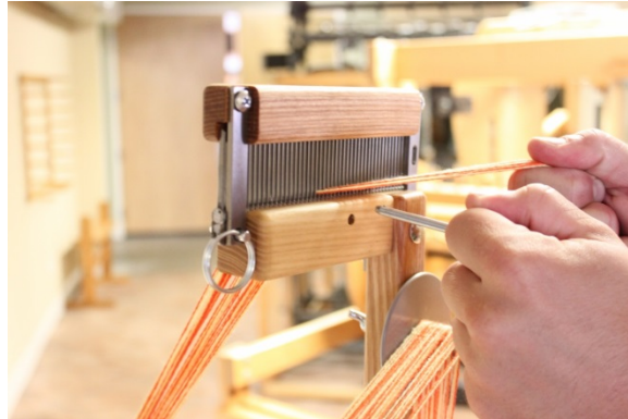
Figure 103 - Remove Raddle from Top Position
