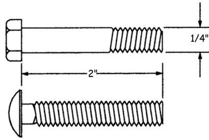
Figure 6 - Measuring Bolts
