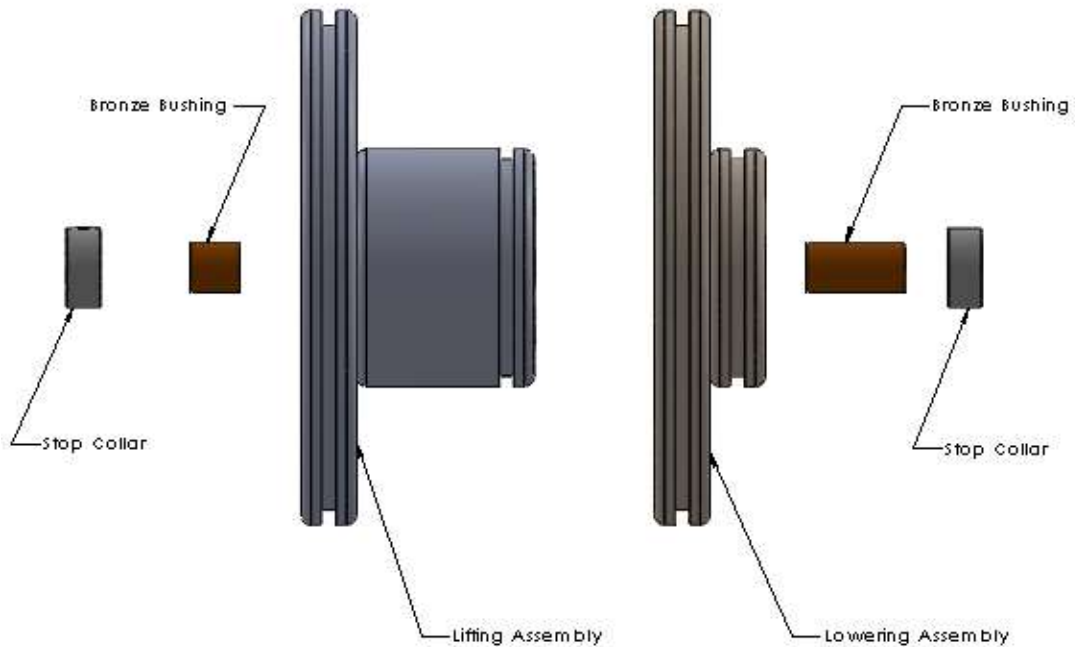
Fig. 3-P – Cam-cylinders Configuration for PDL (right side view)
