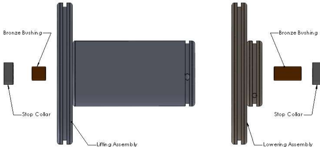
Fig. 3-T – Cam-cylinders Configuration for TDL (right side view)
