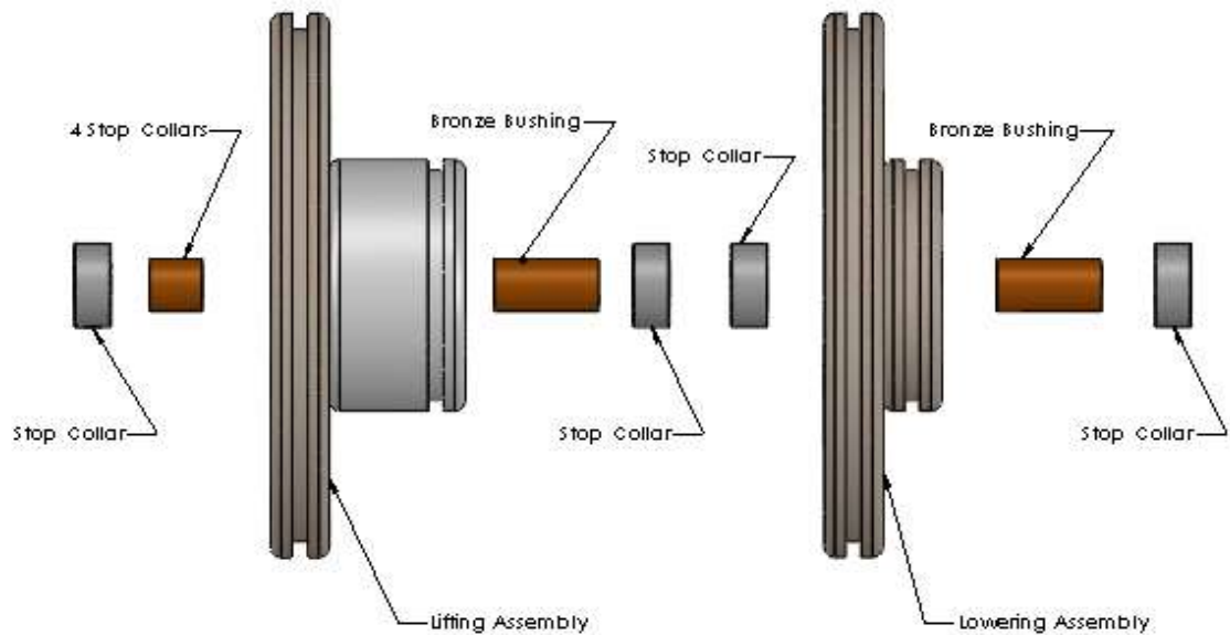
Fig. 3-V – Cam-cylinders Configuration for V-Series (right side view)
