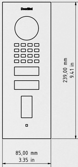
Front panel
