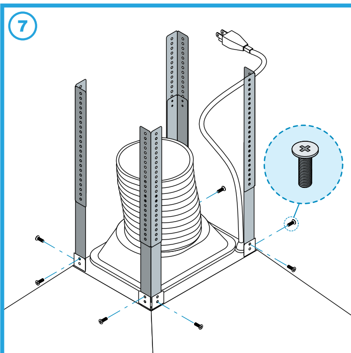
(7) Fasten arm extensions to the unit with screws on each corner.
