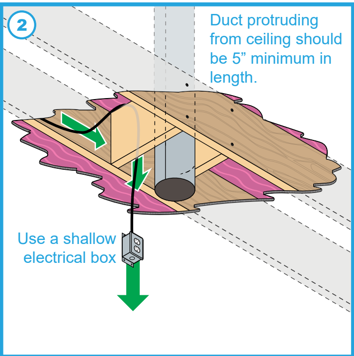
(2) Install an electrical outlet from the ceiling in between the braces. A 8"-Ø duct (10"-Ø optional) to the elbow connection.
