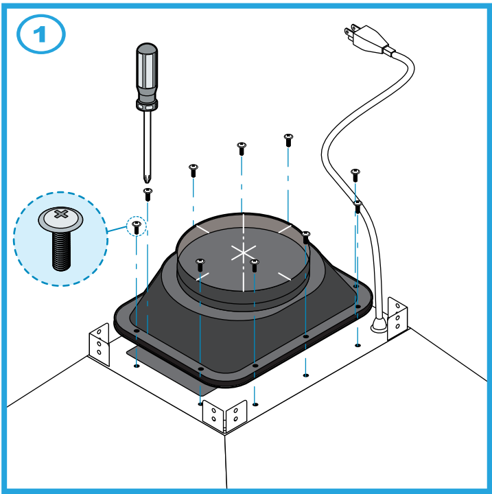
(1) Screw on 8"-Ø transition (10"-Ø optional) to the opening of the fan motor exit.
