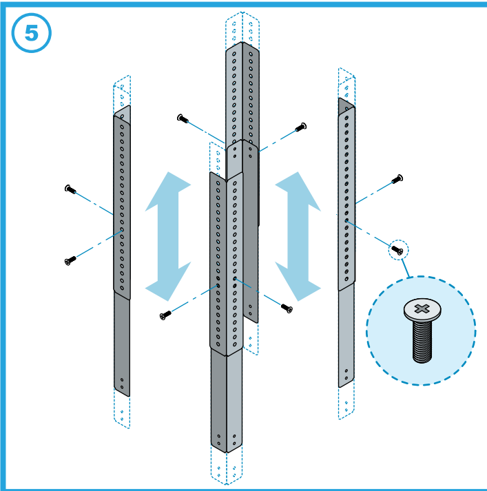
(5) Determine the height needed for the support extensions. Adjust length between the range of 12 ¾" to 23". Secure with screws.
