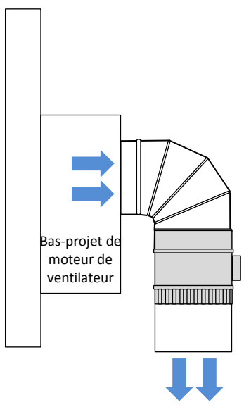
Installation de Downdraft:
