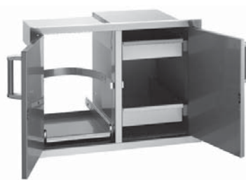
DOUBLE DOORS WITH TANK TRAY & DUAL DRAWERS MODEL: 53930S-12T CUT-OUT: 21" x 30 1/2" x 20 1/2"
