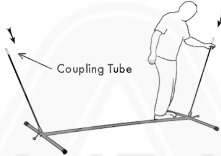
2. Install two lower Black Rods with Coupling Tubes up, in angled Pipes
