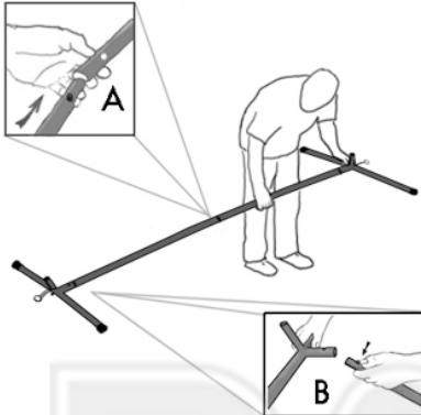
1. Join two straight Pipes together. Fig. A Then attach both end Legs. Fig. B
