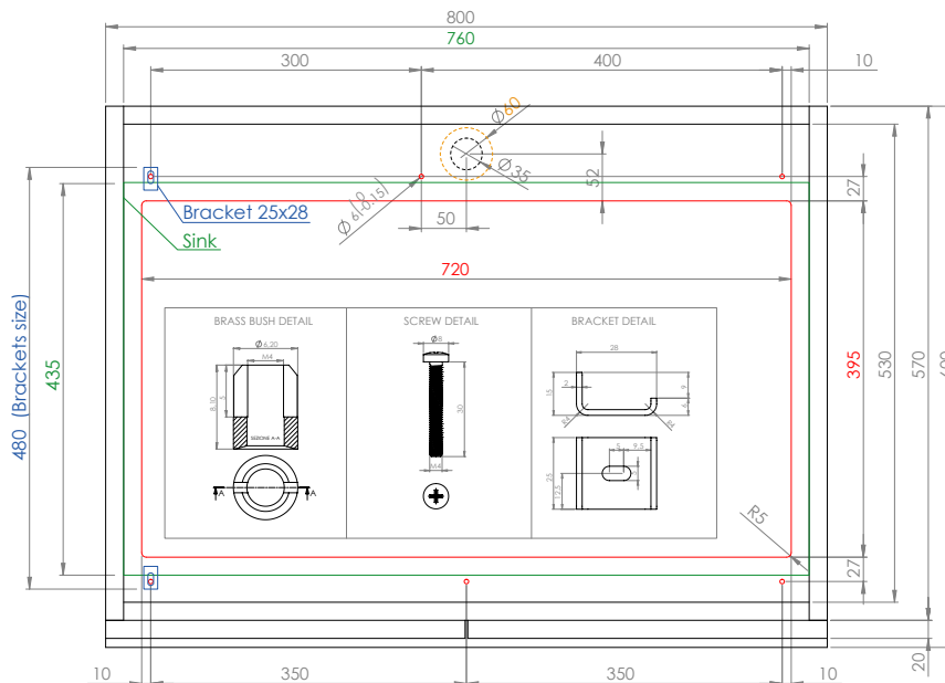
Technical data sheet Quadra 350 Under Mount
