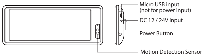
6.8" Motion Activated HD Monitor
