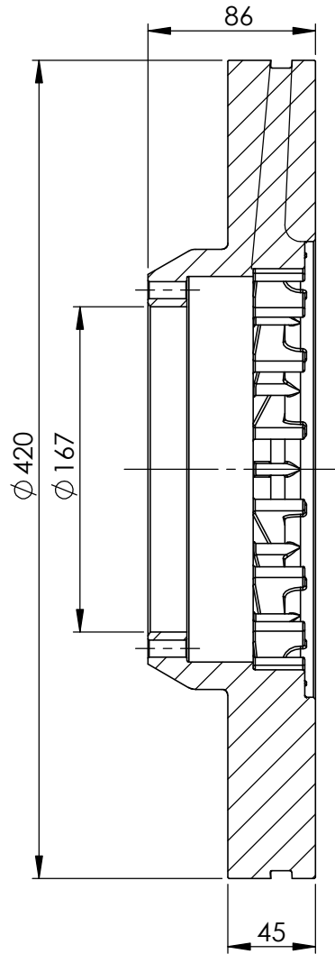
SECTION A-A SCALE 1 : 3.5
