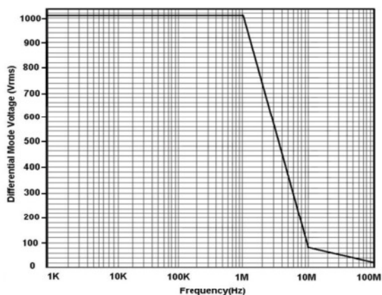
Figure 5 PHA0150/PHA1150 Max. Differential Mode Voltage vs Freq.
