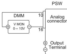
External DMM Monitoring of the Output Voltage
