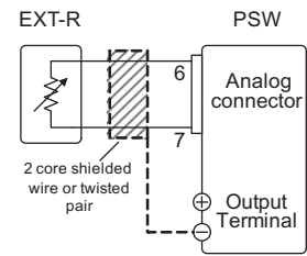
External Resistance control of the Voltage Output
