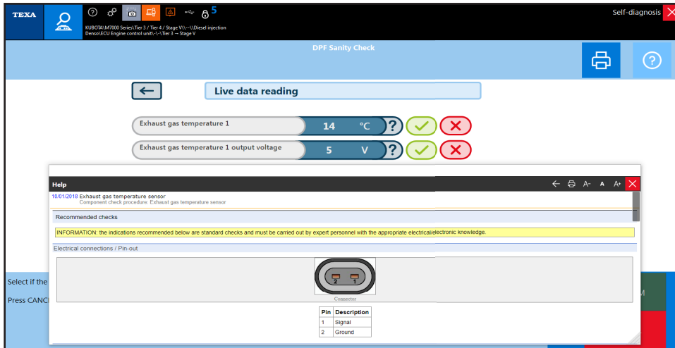
Error parameter reading with help sheet and component sheet.
