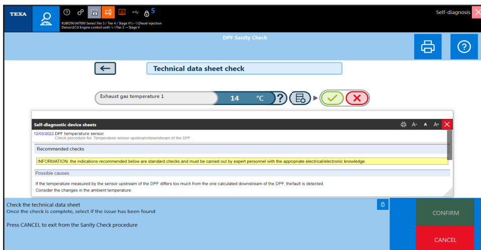
Error parameter reading with technical sheet.
