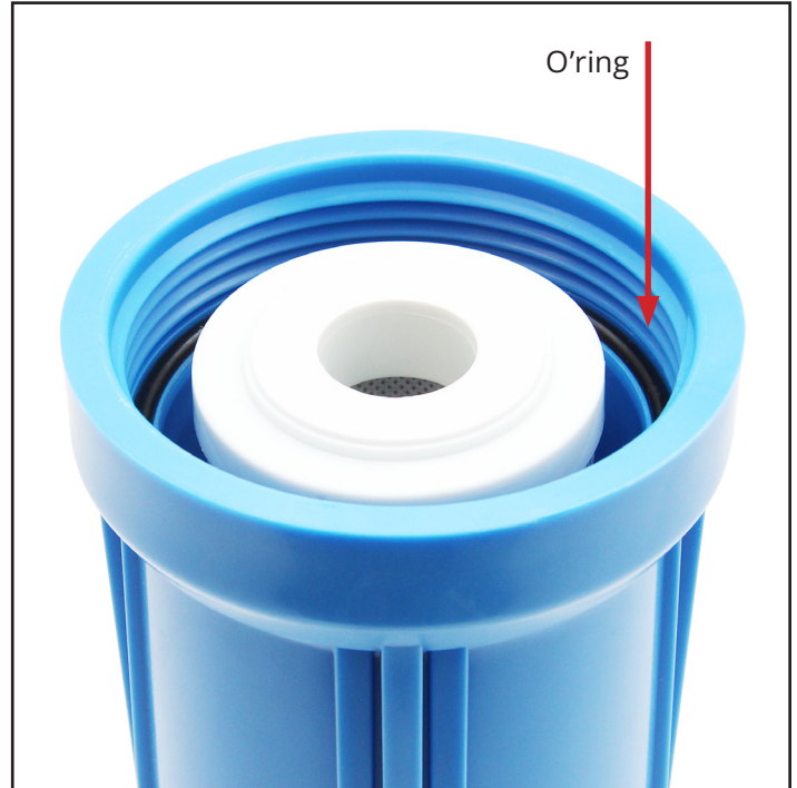
6. Put a carbon filter in the 10 inch housing and make sure the O'ring is in place before install.
