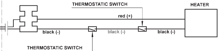
Model: RMD 85x1, 85x5, RML 8551, 8555 OVEN AND WINTER-KIT
