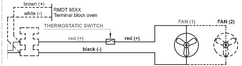
Model: RMDT 85x1, 85x5 OVEN
