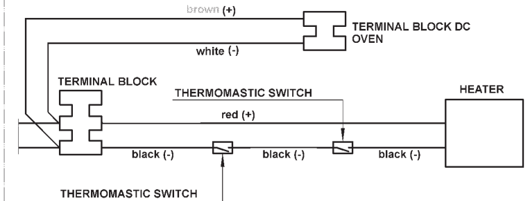
Model: RMD 85x1, 85x5, RML 8551, 8555 OVEN AND WINTER-KIT
