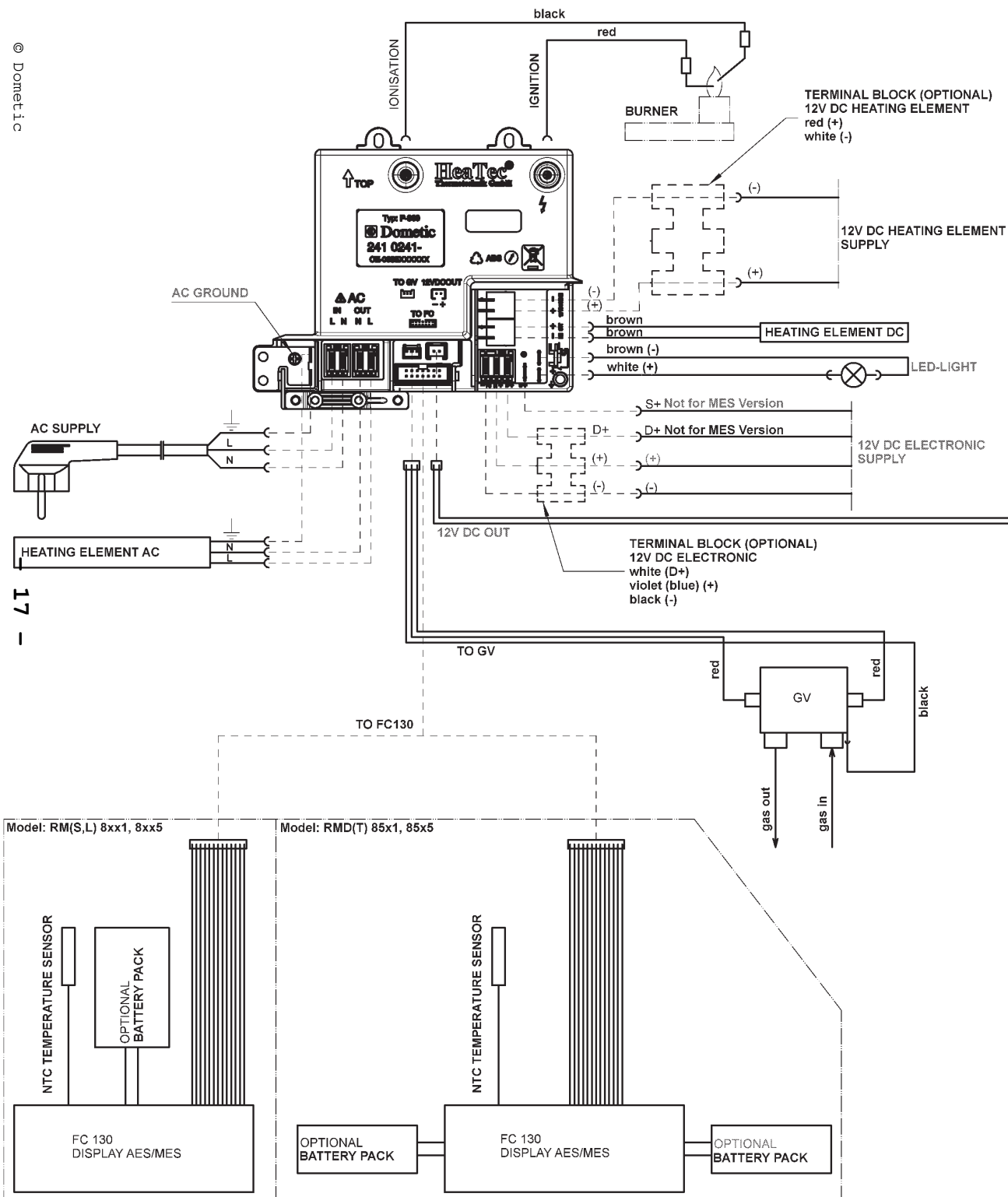
Model: RM(S) 8xx1, 8xx5, RML 8551, 8555, RMD 85x1, 85x5 FAN
