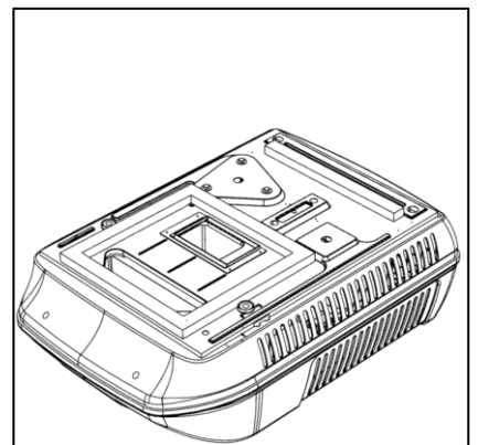
Fig 8: Shows positioning of Spigot to be attached to underside of unit. Ensure spigot is mounted the correct way, screw holes will not line up if attached back to front
