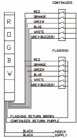
Flash & buzzer type
