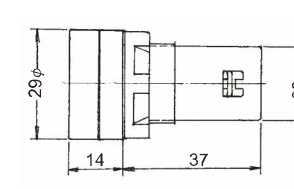
L22, 22 φ LED lamp
