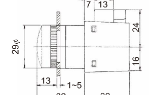
PLT-22 Transformer pilot lamp
