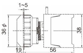
EPFL30-1O/C Push ON-Push OFF
