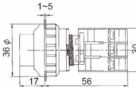
PFL30-1O/C Push ON-Push OFF
