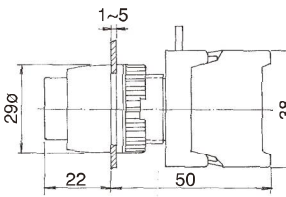
PF22-1O/C Push ON-Push OFF
