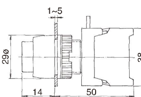
EPF22-1O/C Push ON-Push OFF
