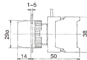
PBL22-1O/C
