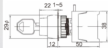
KSR22-2/O 3 Position 1-0-2 Spring return KSR22A-2/O 1-0-2, KSR22B-2/O 1-0-2
