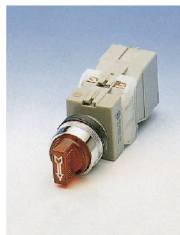
TUSS 22-1O/C, 1-2 SPRING RETURN TUSS 22-2/O, 1-0-2 SPRING RETURN
