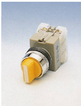
LUSS 22-1O/C, 1-2 SPRING RETURN LUSS 22-2/O, 1-0-2 SPRING RETURN
