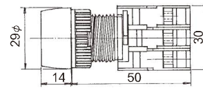
GEPFL22-10/C Push ON-Push OFF
