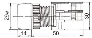
GLBL22-10/C
