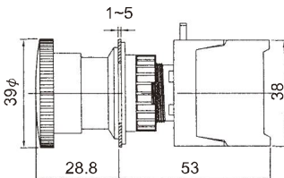
MBL22-10/C Illuminated latching stop
