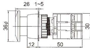
MBL22-1/C Illuminated latching stop
