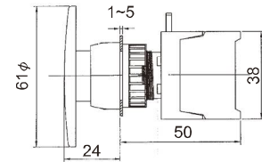
GPFL22-10/C Push ON-Push OFF
