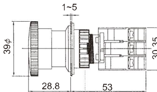
MBL22-10/C Illuminated latching stop
