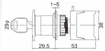
EKS22-1/O Emergency stop key switch EKS22-10/C
