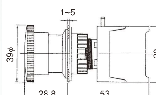
Latching stop
