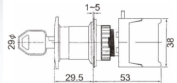
EKS22-1/O Emergency stop key switch EKS22-10/C
