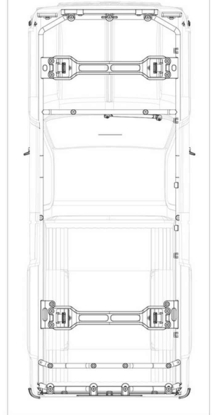
Completed Assembly (view from bottom)
