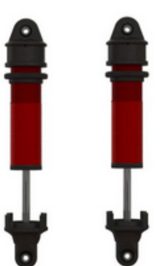
ARA330749 SHOCK SET BORE:20MM, LENGTH:188MM, PISTON:8X1.5MM,...
