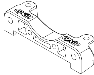
ARA330647 - Lower Suspension Hanger Front Rear CNC 7075 T6 Aluminum
