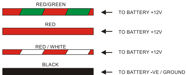
Figure 8 - Battery Wiring
