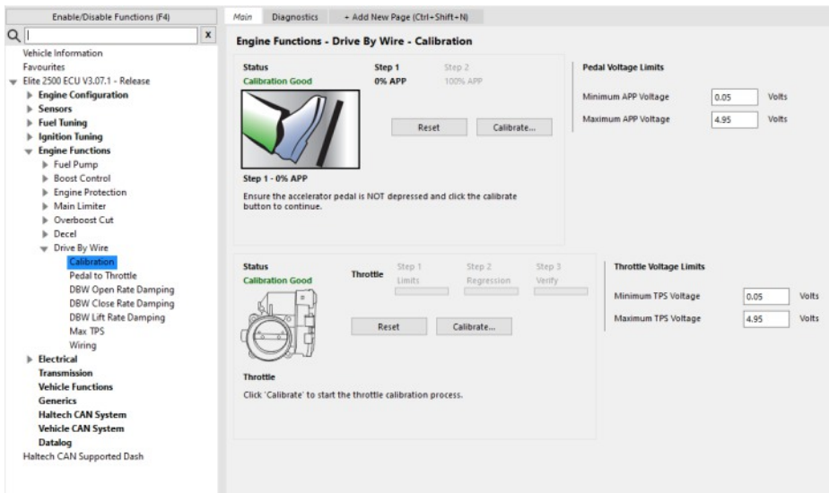
Figure 9 - DBW Throttle Calibration
