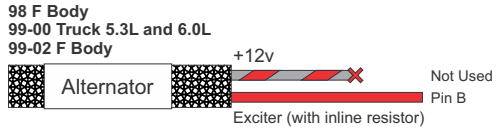
(Looking into connector, pin side) Supplied Alternator Connector
