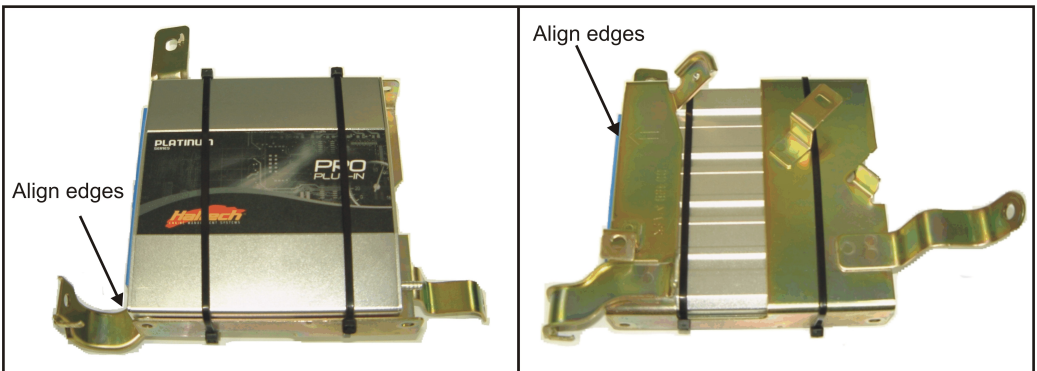
Figure 3 – Haltech ECU Mounted to Factory ECU Mount
