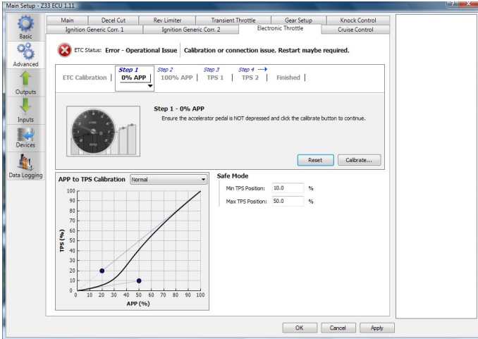
Figure 10 – 0% APP Successful calibration display
