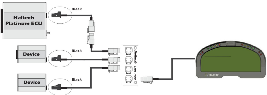
Figure 18 – Haltech ECU connected to 3 Auxiliary CAN based devices
