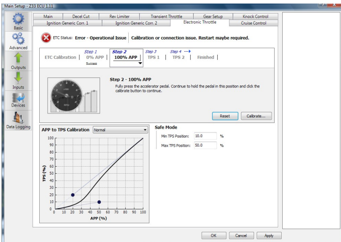
Figure 11 – 100% APP Successful Calibration display
