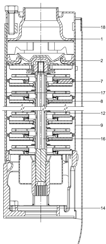
Example SP 3A, pump with spline shaft.
