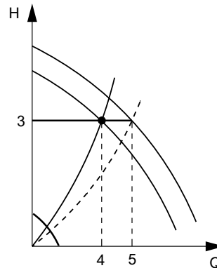
Constant pressure control
