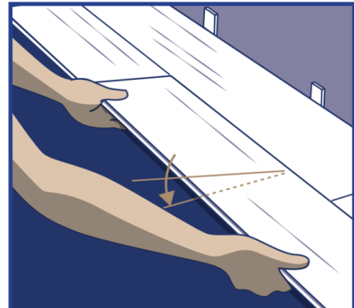
Step 4: Lock long edge of plank by inserting tongue into groove at an angle and drop in place. Slide plank toward end of previously installed plank until the tongue just touches the groove.
