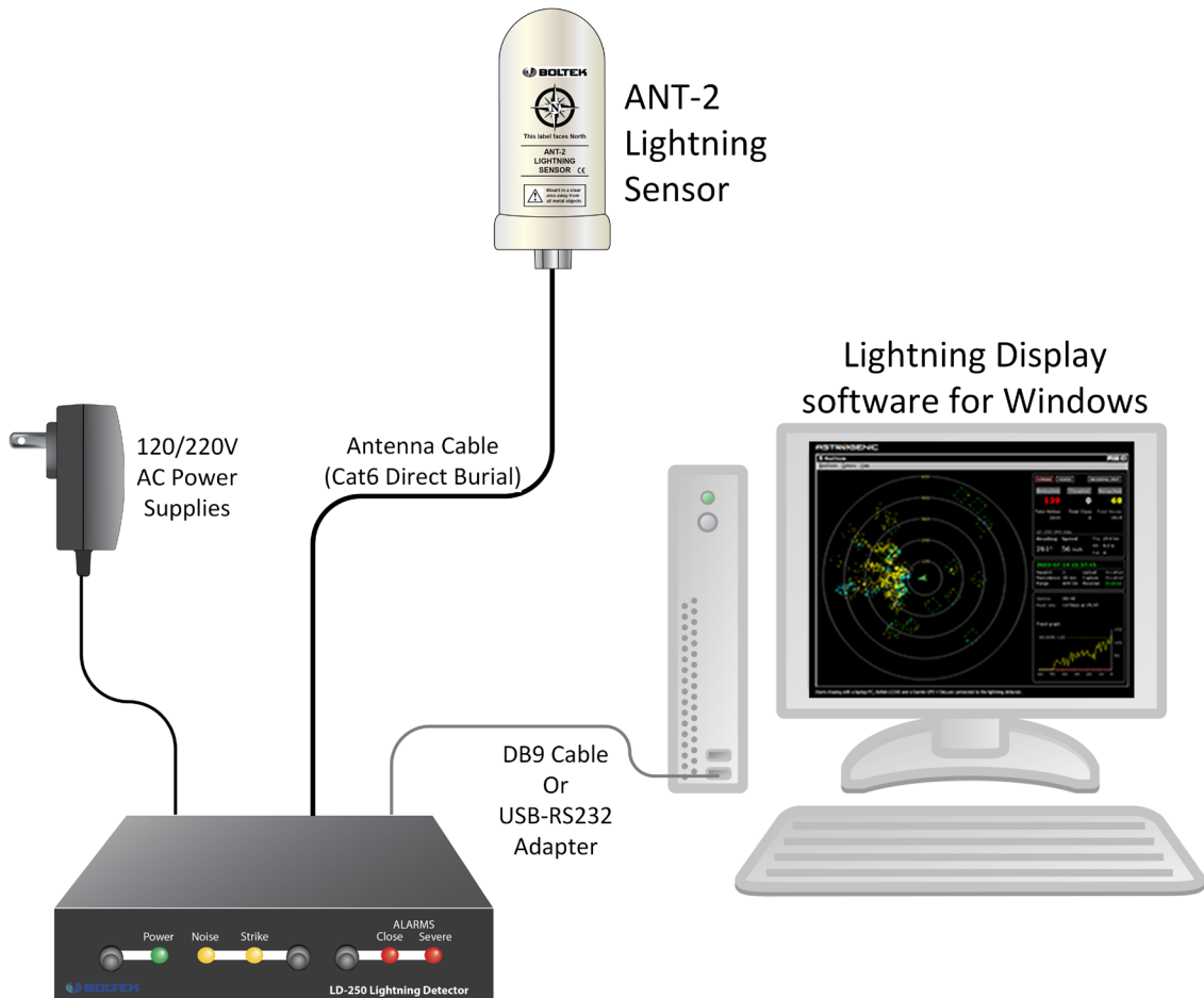
LD-250 Connection Diagram
