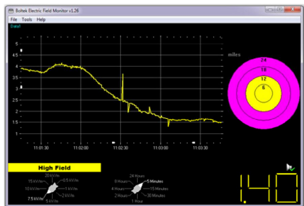
Lightning and high field alarm active
