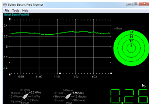
EFM-100 Electric Field Monitor Software (included)
