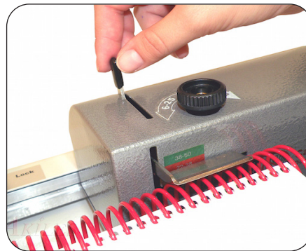
Adjustable side guides
