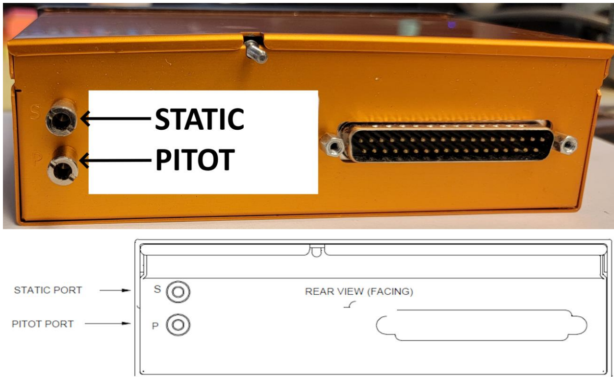
FIGURE 2 – PANEL MOUNT PN: 20000000
