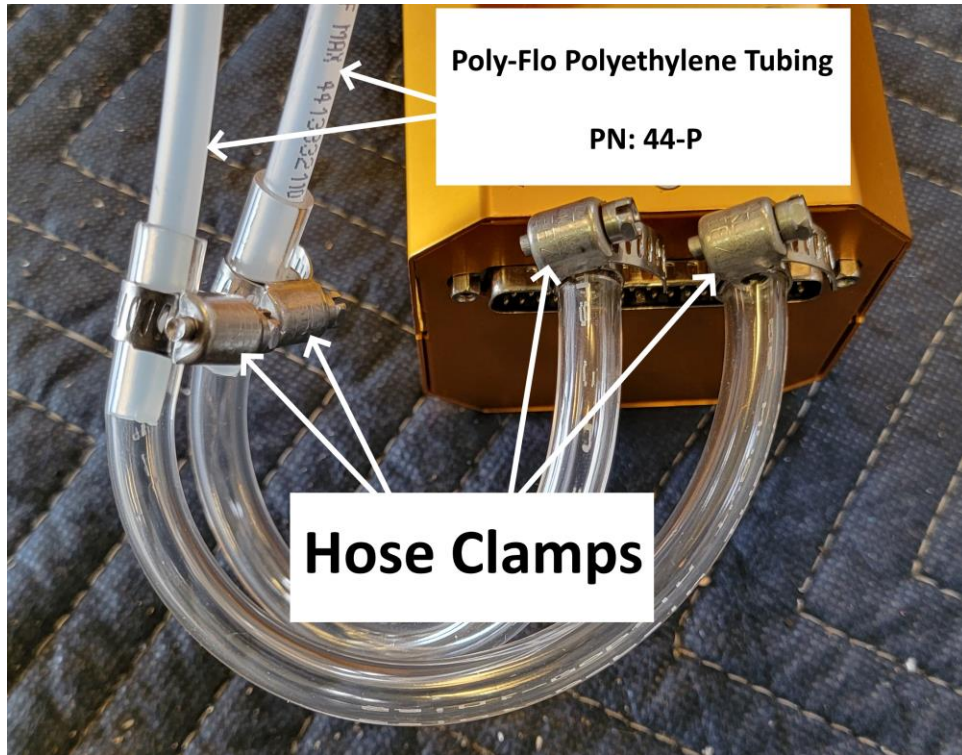
FIGURE 5 – POLY-FLO TUBING & HOSE CLAMPS
