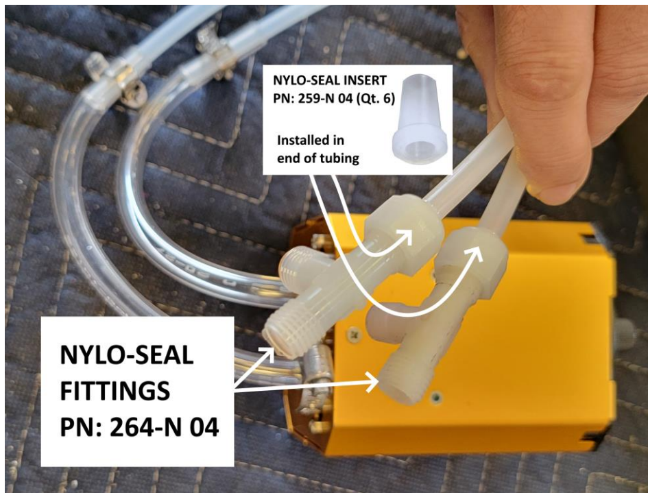
FIGURE 6 – NYLO-SEAL T'S & INSERTS
