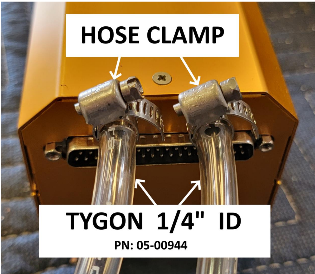
FIGURE 4 – TYGON & HOSE CLAMPS
