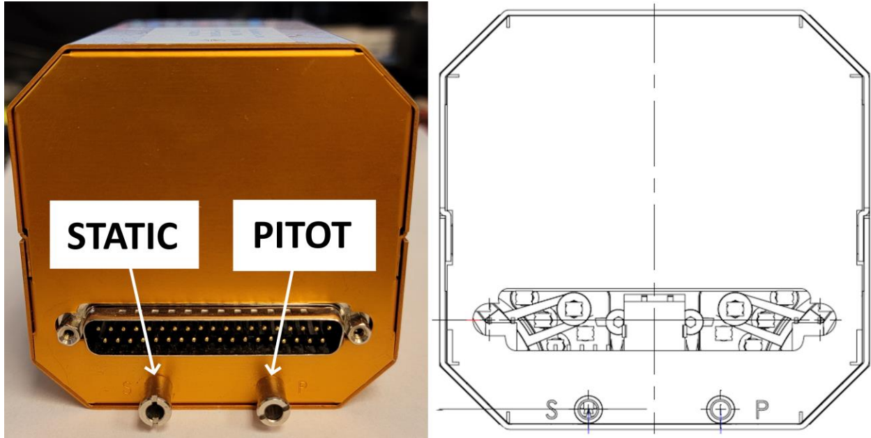
FIGURE 1 – INSTRUMENT MOUNT PN: 10000000
