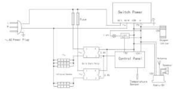
Circuit Diagram B
