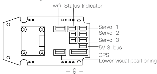
Flight Control Interface Diagram
