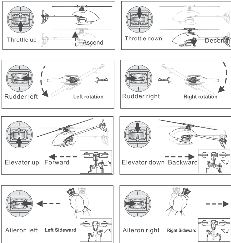
Flight Control Interface Diagram
