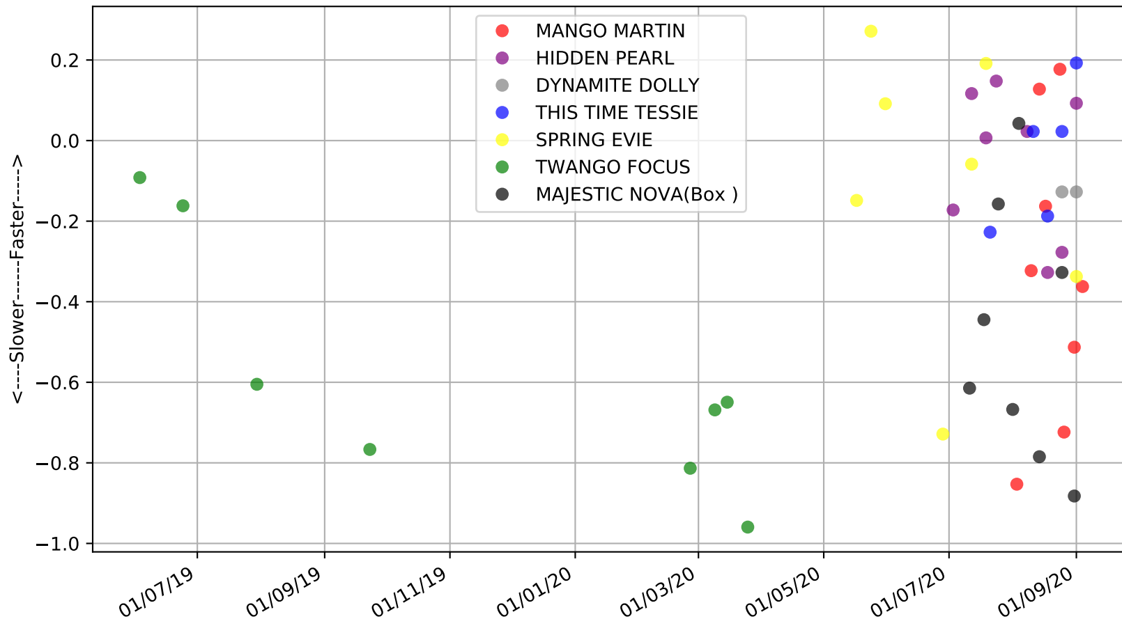
Ipswich - 8th Sep Race 2, SKY RACING, 431m, MH Speed of dog compared with par win times of the track & distance it ran at
