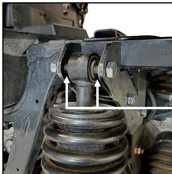
3/8" LG. SPACERS
