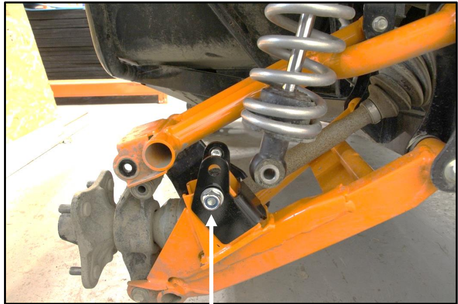
M12 Washer and M12 Lock nut
