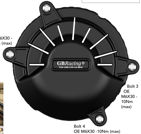
FIG 1. ALL 4 BOLTS SHOWN HERE ARE THE ORIGINAL BOLTS
