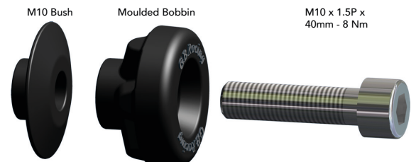
M10 Bush
