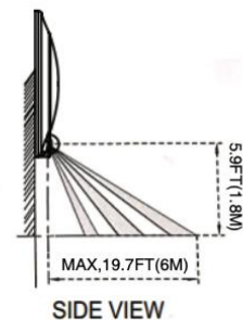
Wall Mount sensor Detection Range
