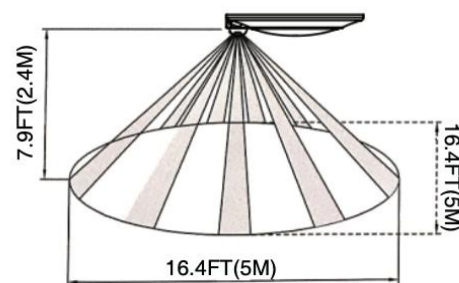
Ceiling Mount sensor Detection Range
