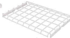
Wireguard
