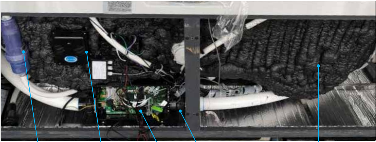
Ozone Mixing Chamber Ozone Generator Control pack Heater Black out insulation
